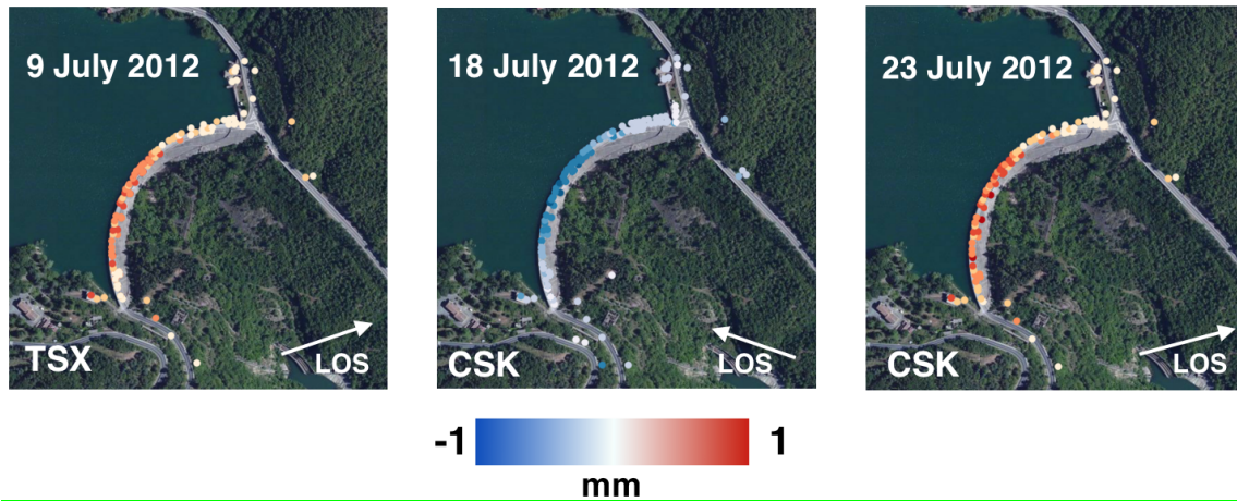
Figure 6: Cumulative displacement maps at the Pertusillo dam as observed from different sensors and different look geometries. Negative values indicates motion away from the satellite. Optical image from Bing Maps.
