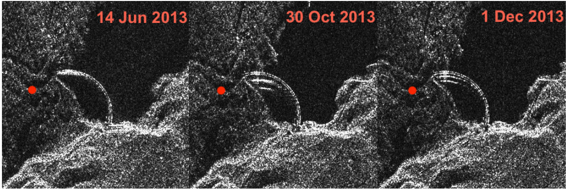
Figure 4. Double bounce effect recorded during different periods of the year affecting the CSK ascending. The descending dataset does not show this effect. Reference point used for PS-InSAR analysis showed in red.
