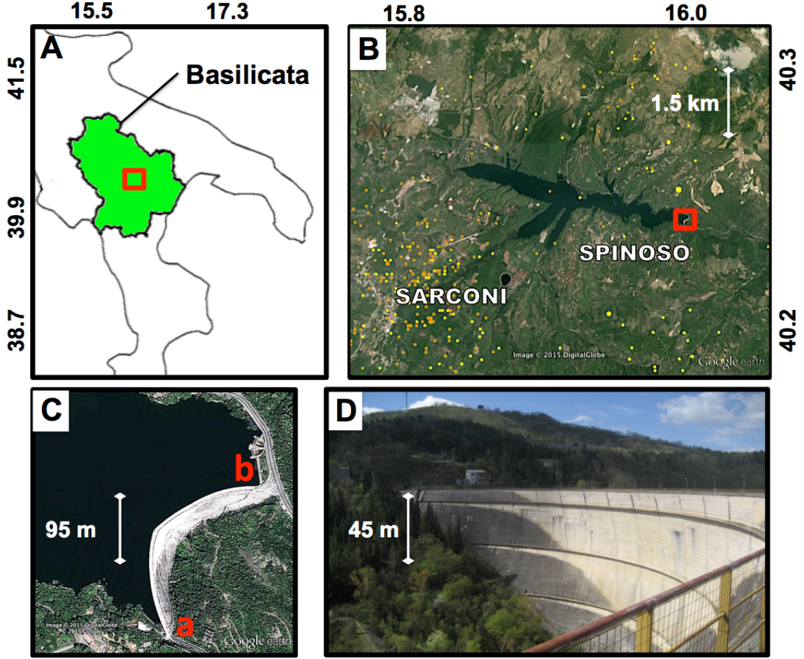
Figure 1 Overview of the study site (A) South Italian Peninsula; the red outline shows the extent of the Pertusillo artificial lake in B. (B) Google-Earth Optical Image showing the “Lago di Pietra del Pertusillo”. Seismicity at the Pertusillo dam recorded by the ISIDE-INGV network. Yellow (orange) dots indicates earthquakes with 0-10 (10-20) km depth The red box shows the extent of the dam in C. (C) Google-Earth optical image evidencing the sides of the dam (D) side view of the dam. Scale bar is referenced to the height of the dam.
